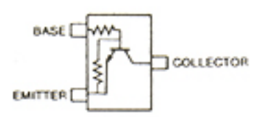
DTC114EU (Symbol: 24)
